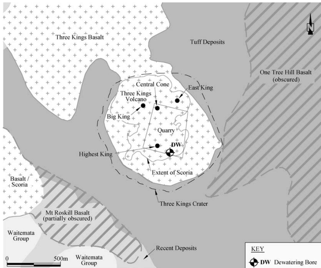
Figure 2. Three Kings geology
